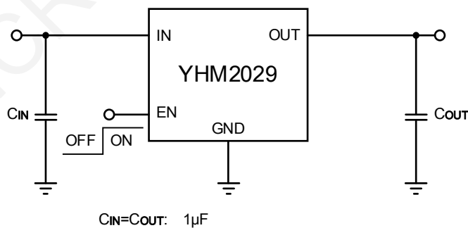
Figure 1. Application Diagram
