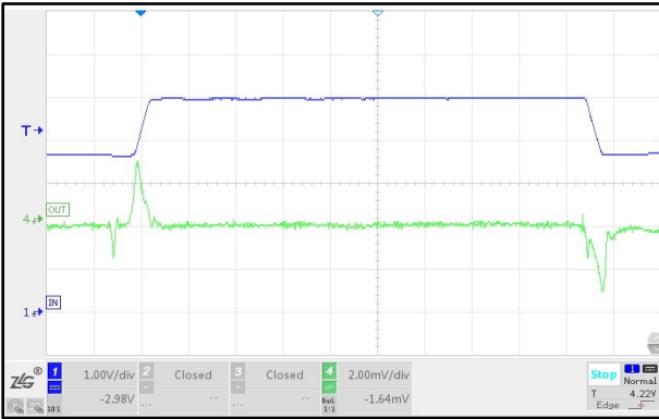
Figure 12. Line Transient ( I_{OUT}=200mA )
