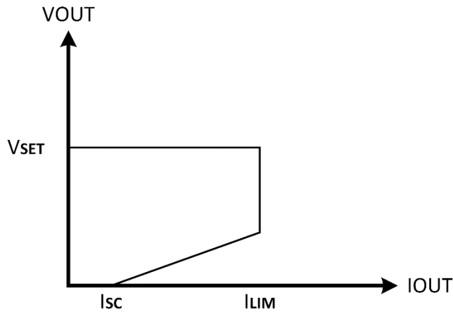
Figure 20. OCP behavior
