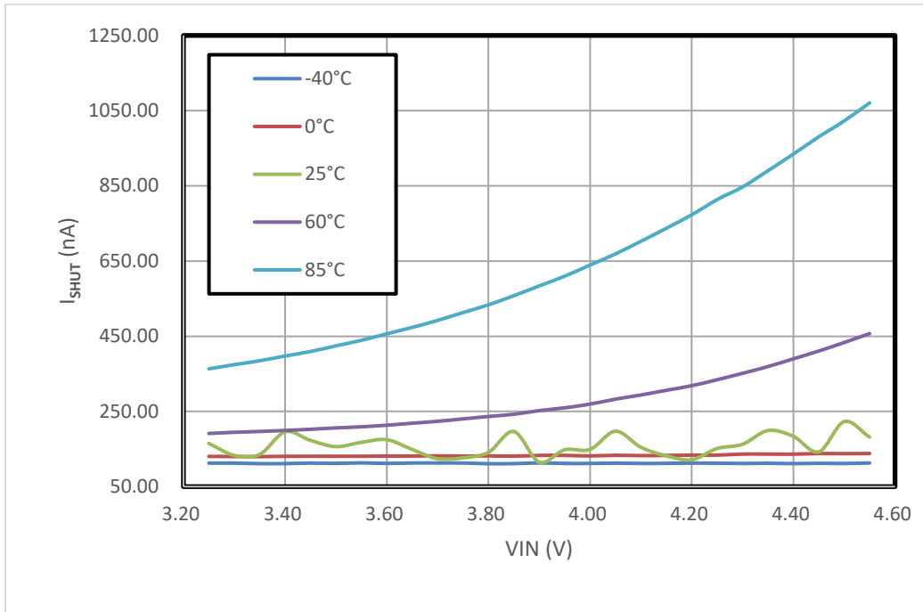
Figure 15. I SHUT vs V IN (V SET = 3.3V)
