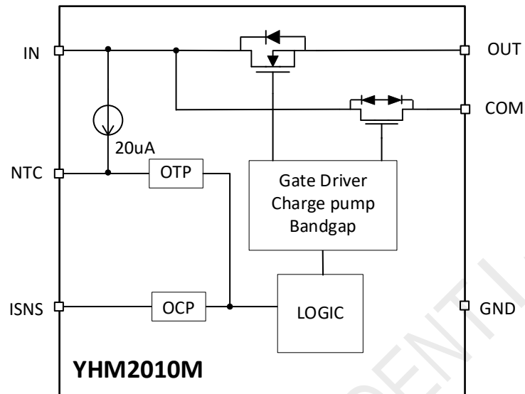
Fig 2. YHM2010M Functional Block Diagram
