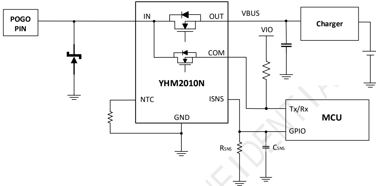
Fig 1. POGO Pin Communication and OVP Application Diagram
